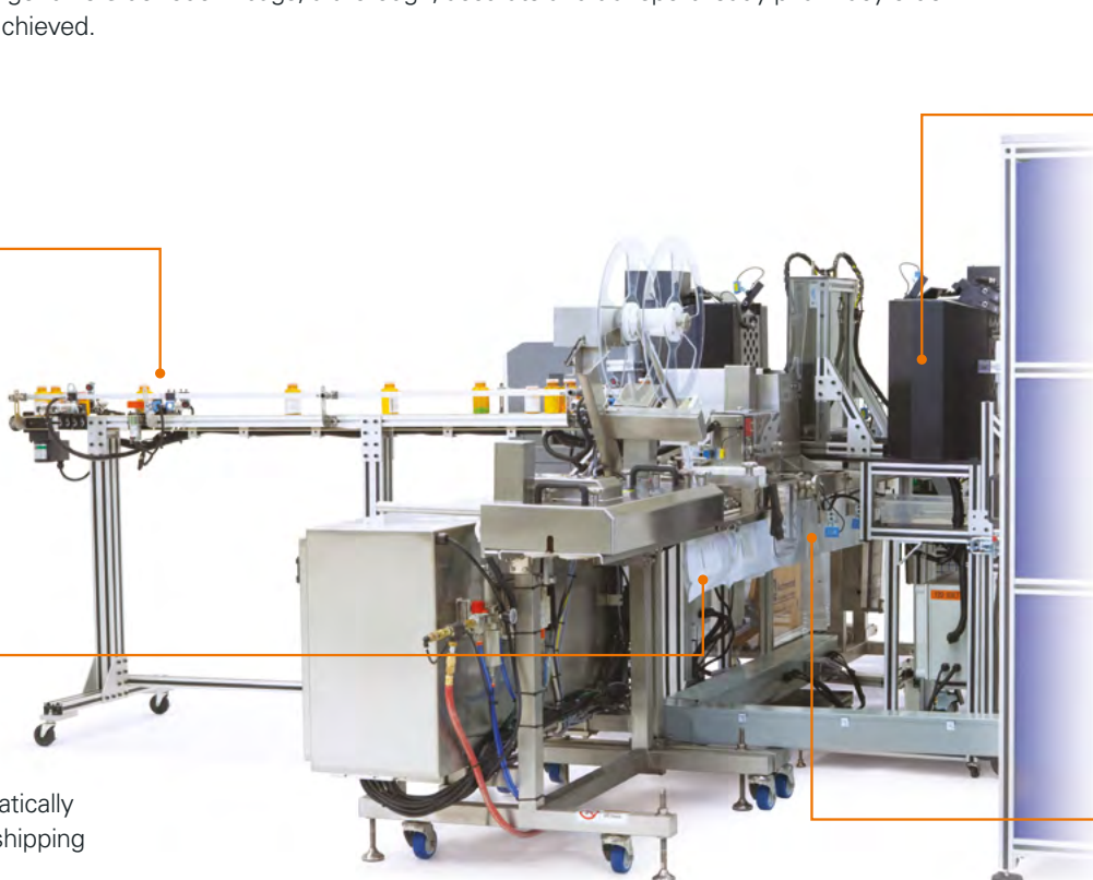
Patient information inserts are automatically printed, indexed, verified, folded and inserted with the integrated Continuous Print System
